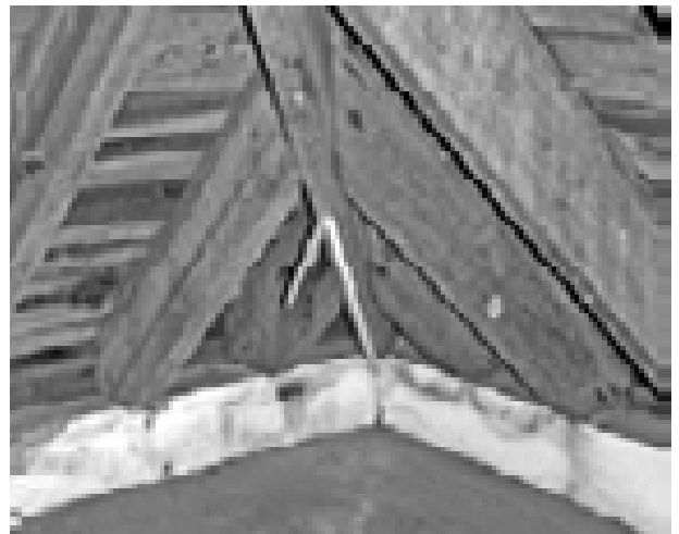
FIGURE 65. View of roof hip and junction of rafters and top plate of second floor walls. (T. Jones, NPS, 2005)
