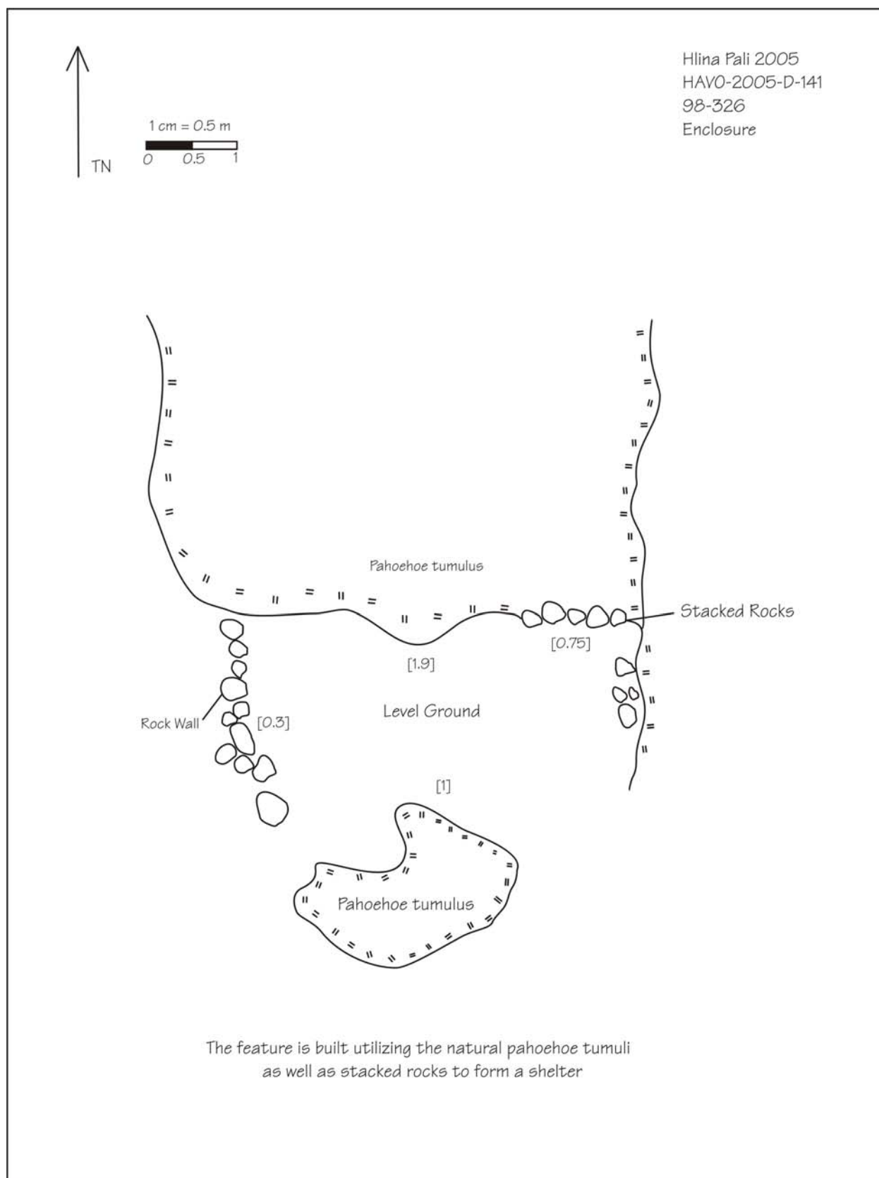
Figure 73. HAVO-2005-D-141, Enclosure
