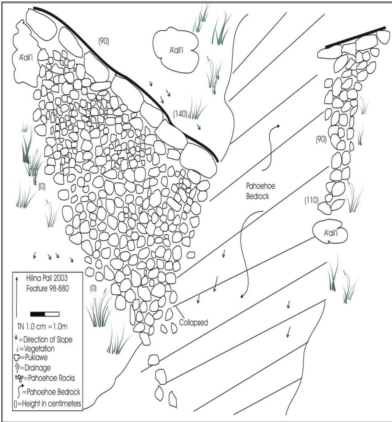
Figure 48. Feature HAVO-2005-D-56, Dam
