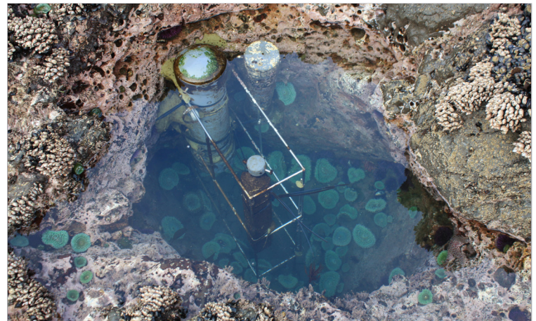
The OA monitoring instrument package installed in a tidepool at Sokol Point, OLYM. This package includes newer SeaFET™ instrumentation (inside cage), and the Collocated older multiprobe datasonde that will be phased out in 2017. NPS Photo
