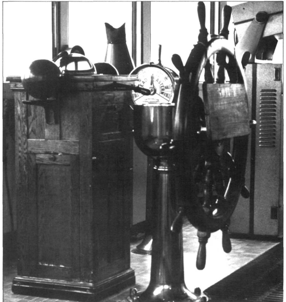
FIGURE 14: The assembly of instruments in the pilot house of the S.S. Clipper represent the various navigational technologies used on the vessel during her career. Documentation of a vessel for the National Register should include views which interpret changes or alterations. (Photo credit: Harry Weese and Associates)
