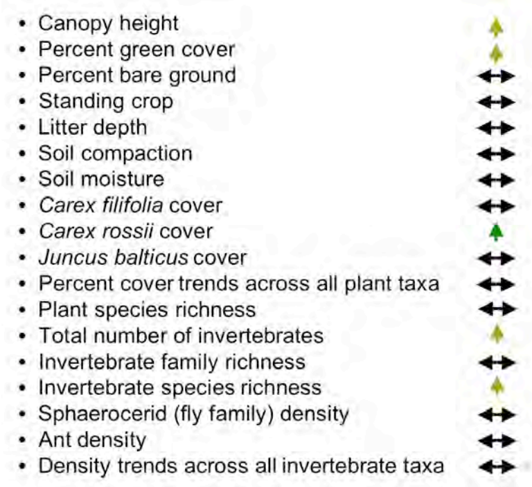
Fig. 34. Summary of 2006 changes on trampling enclosure plots. Upward facing arrows indicate an increase for a given metric, there were no decreases. The double-headed horizontal arrows indicate no change. The dark green arrow represents a strong positive effect, and the light green arrows represent weak positive effects.
