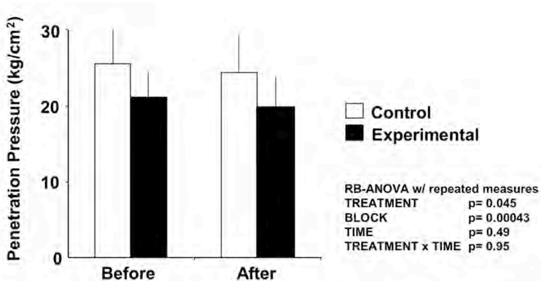
Fig. 29. Mean (SE) penetration pressure on control and enclosure plots before and after the 2006 experiment. BLOCK represents plot effects. n= 10.
