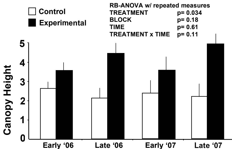
Fig. 35. Mean (SE) canopy height on control and enclosure plots 2006-7. BLOCK represents plot effects.
